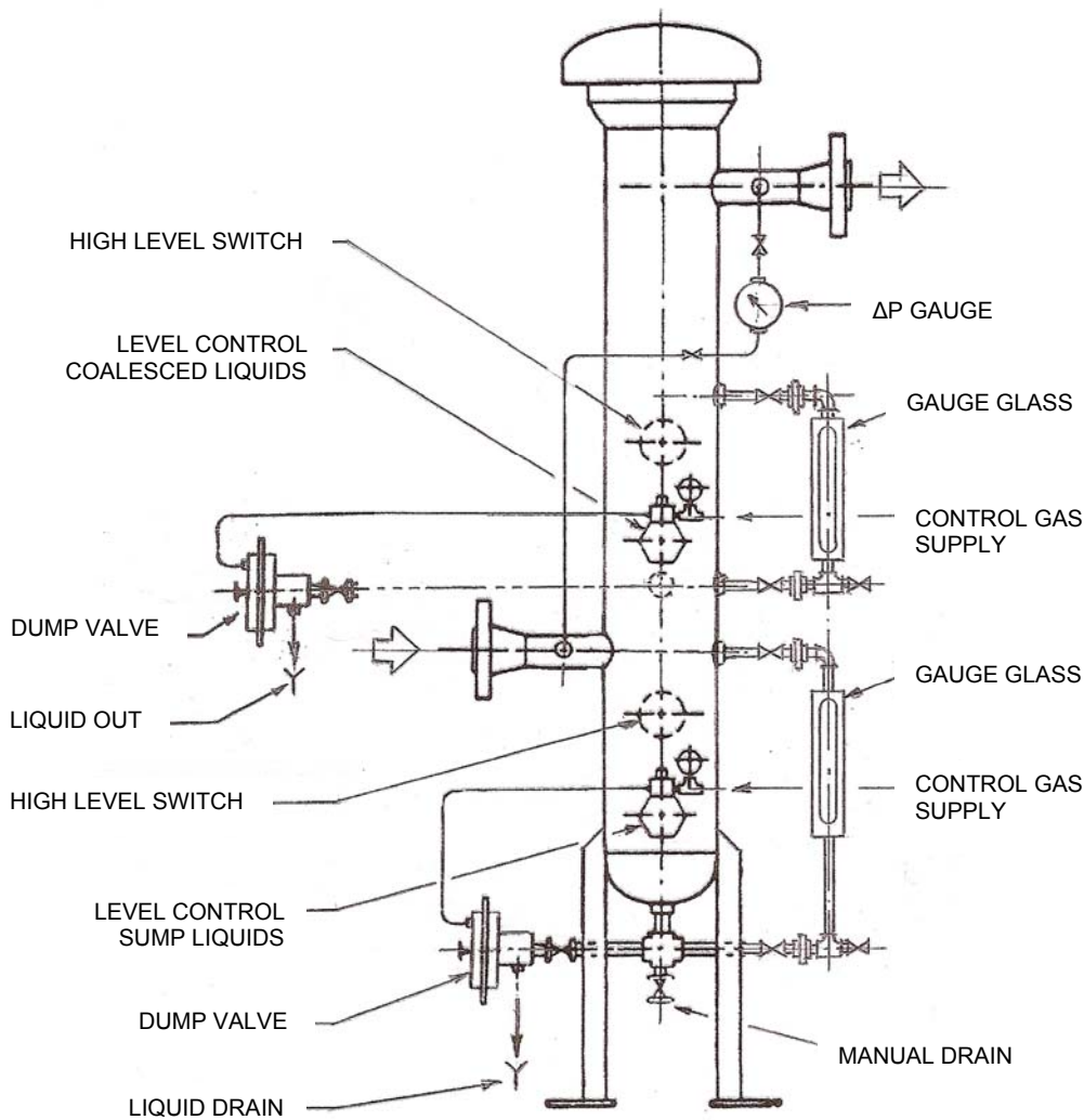
COALESCER WITH LEVEL CONTROLS
